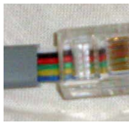
Bad Crimp
