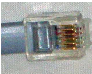
Good Crimp
