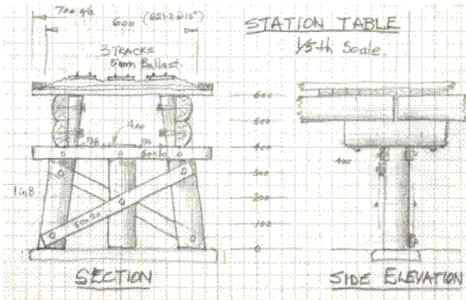
Sketch of the trestle Bents.
